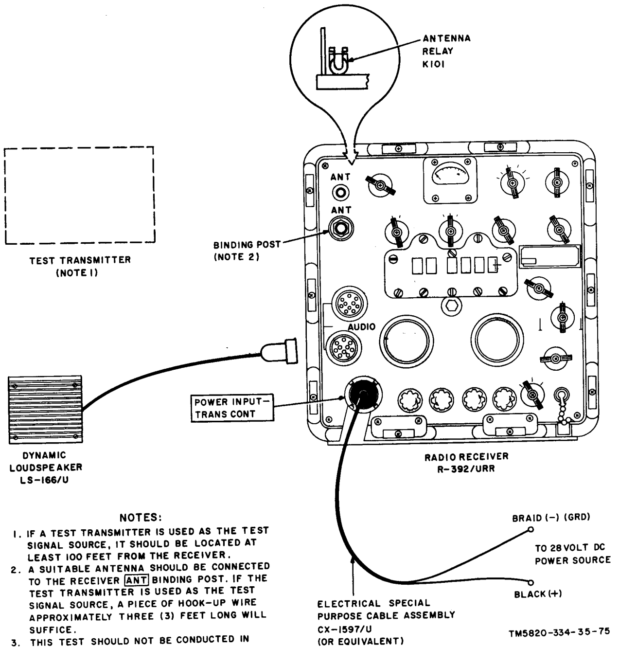
Figure 75. Operational test.
