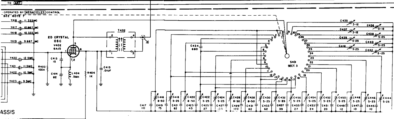
radio receiver, wiring diagram (part 1 of 2).
