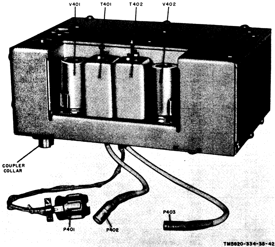
Figure 45. Crystal oscillator subchassis, bottom view.
