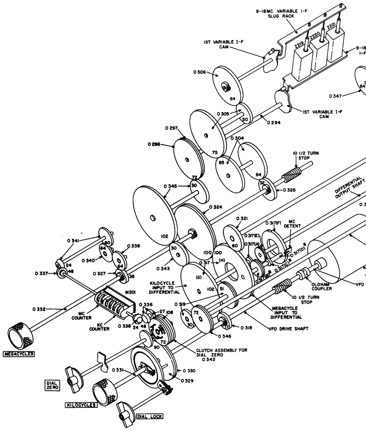
Figure 31. Tuning system
