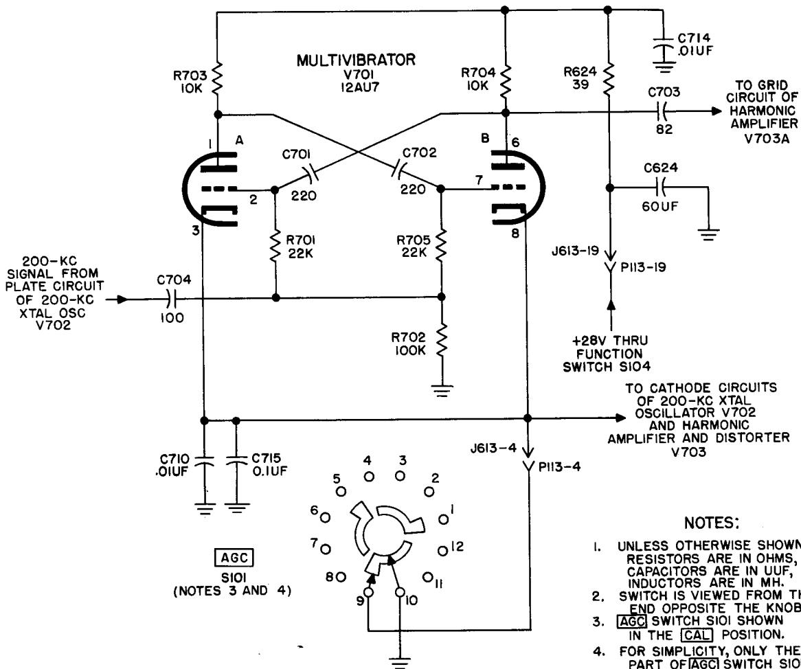
Figure 23. Multivibrator V701, simplified schematic diagram.
