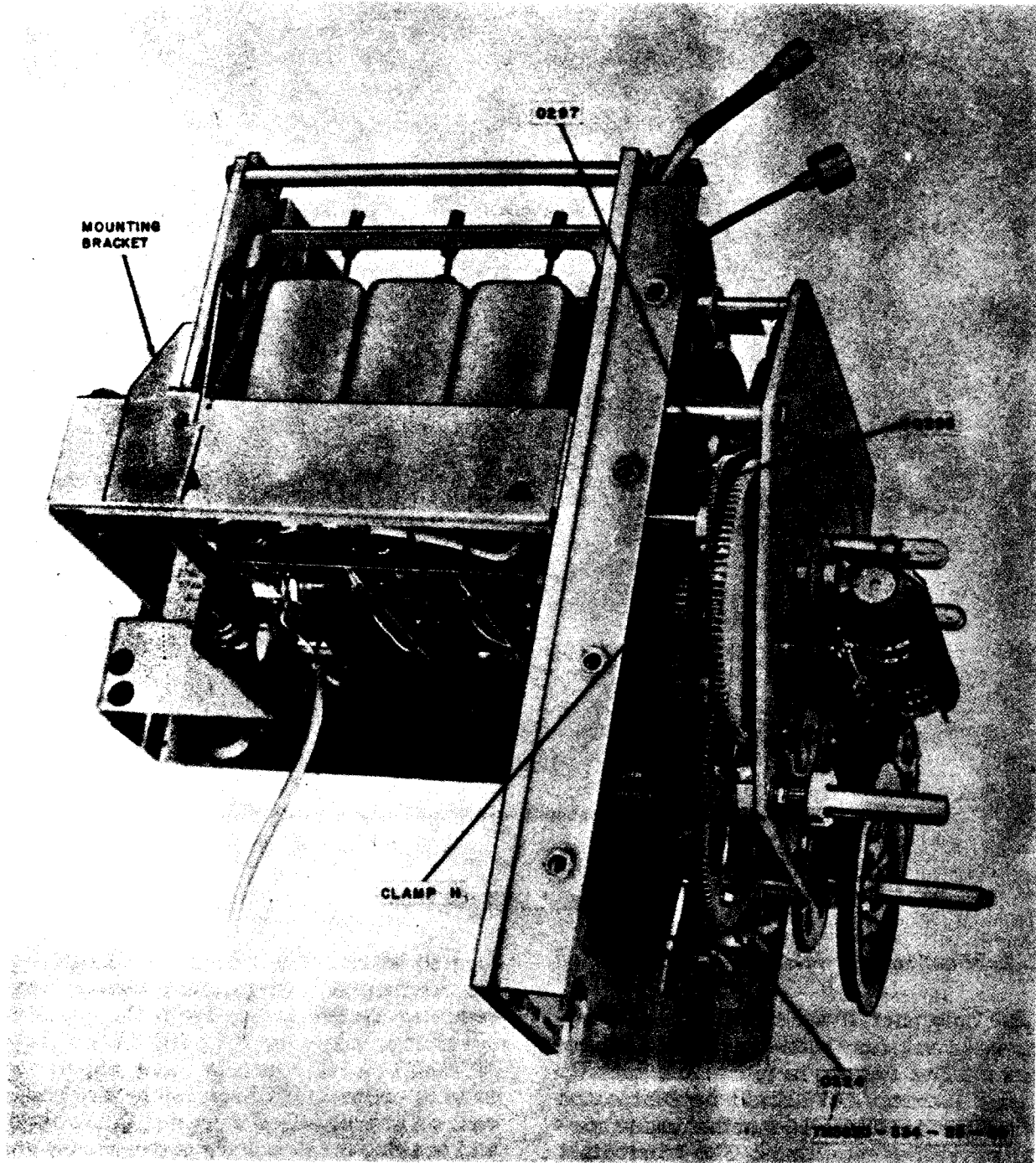
Figure 61. Gear train assembly and rf subchassis, left view.
