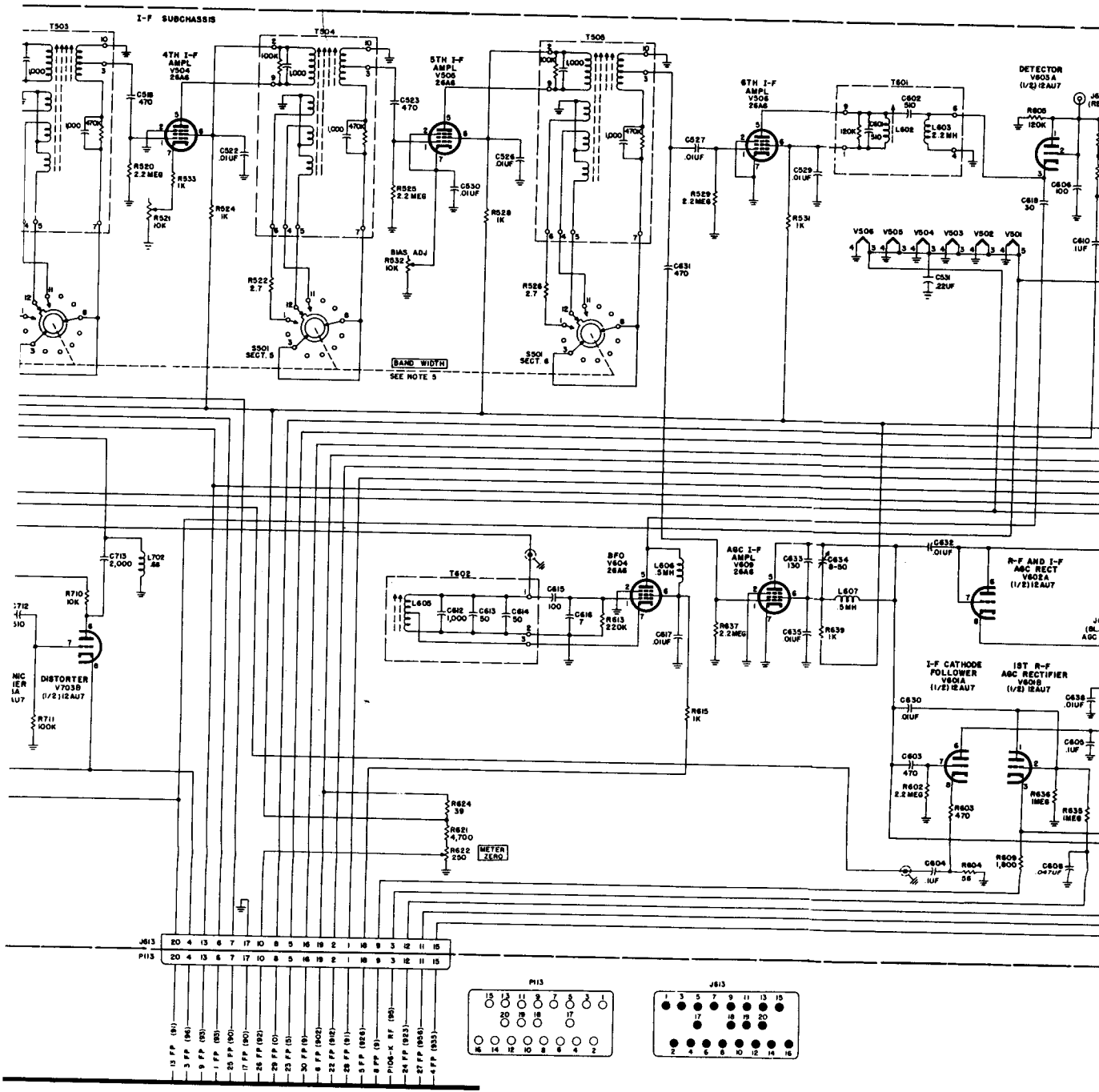
radio receiver, wiring diagram (part 2 of 2).
