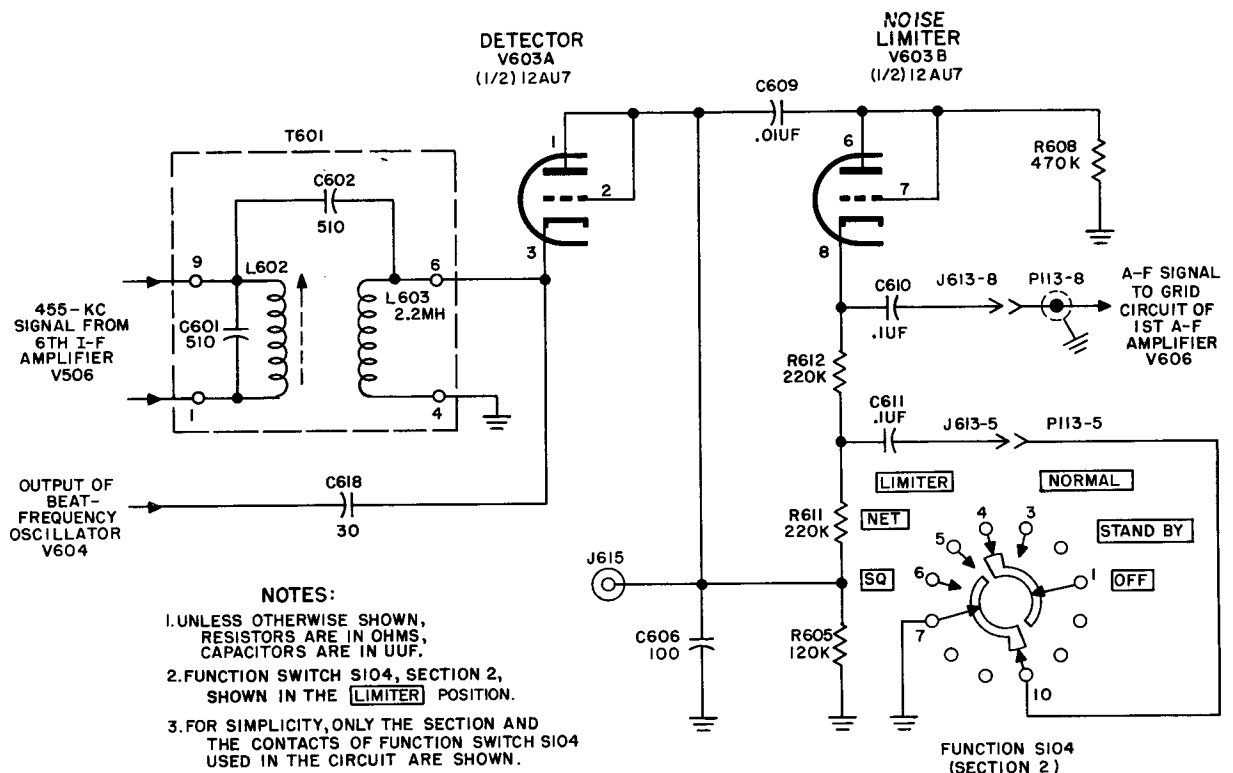
Figure 12. Detector and noise limiter, simplified schematic diagram.
