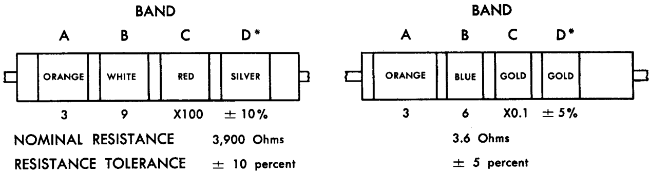
Figure 76. MIL-STD resistor color code markings.
