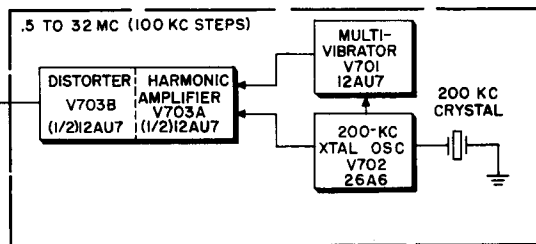
CALIBRATION-OSCILLATOR SUBCHASSIS
