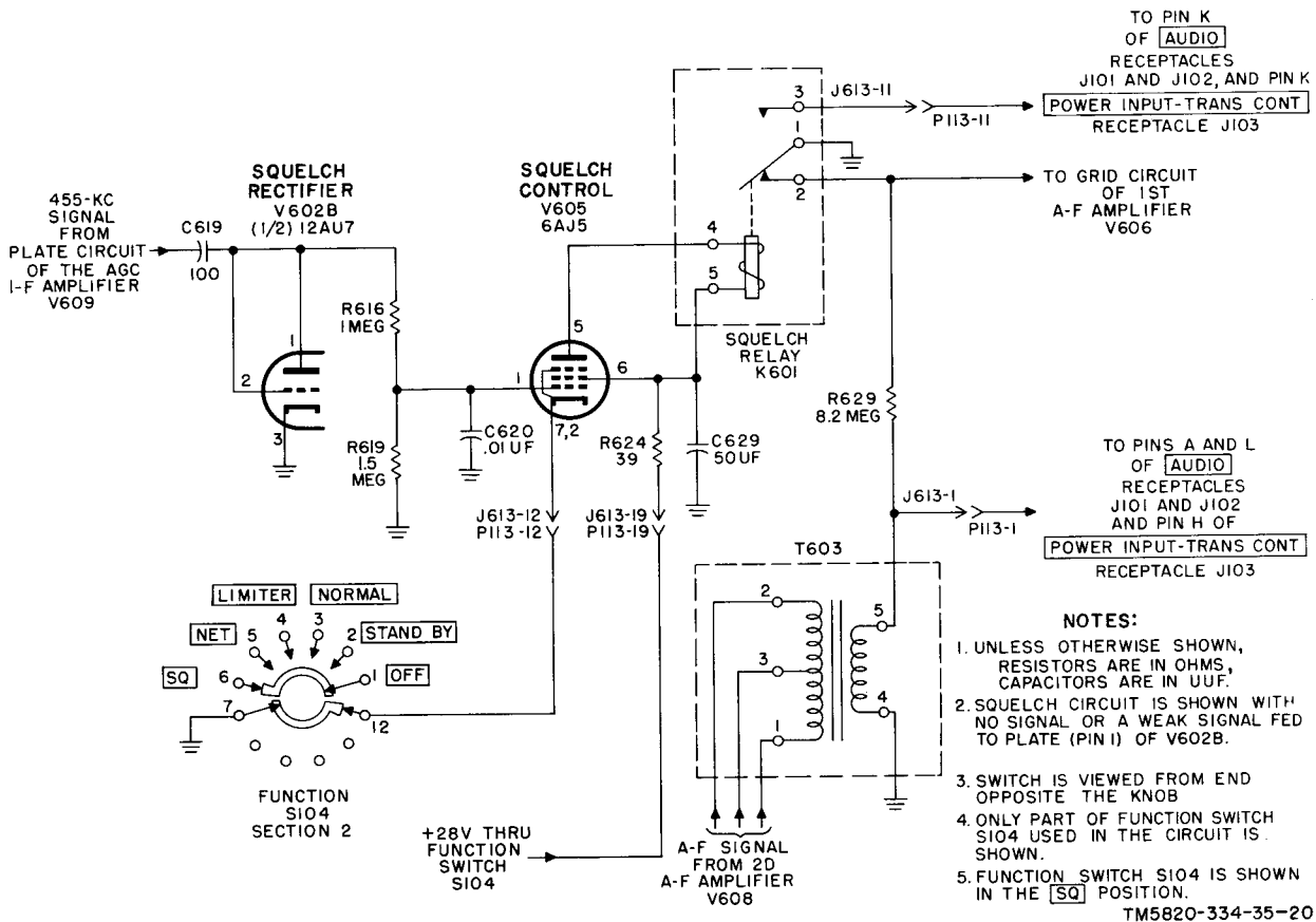
Figure 21. Squelch circuit, simplified schematic diagram.
