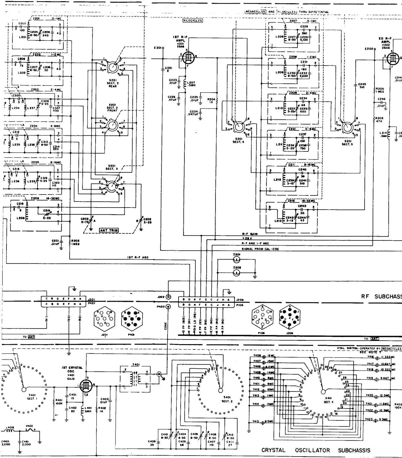
Figure 82(1). Radio receiver, wiring
