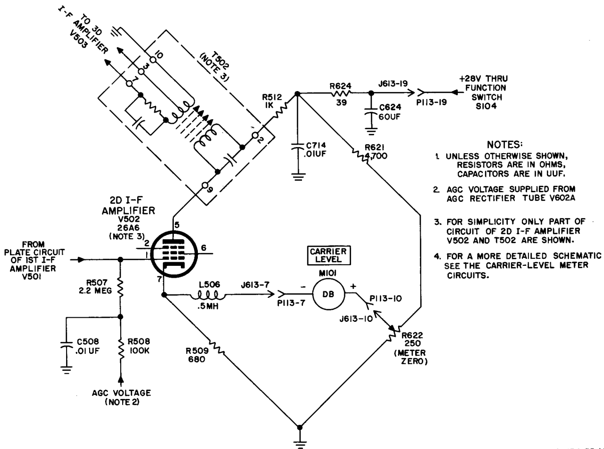
Figure 16. CARRIER LEVEL meter circuit, simplified schematic diagram.
