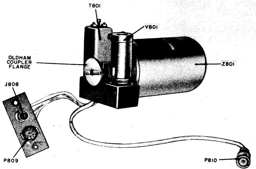
Figure 41. Vfo subchassis.
