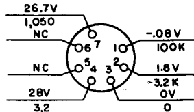
1ST MIXER 26C6 V203
