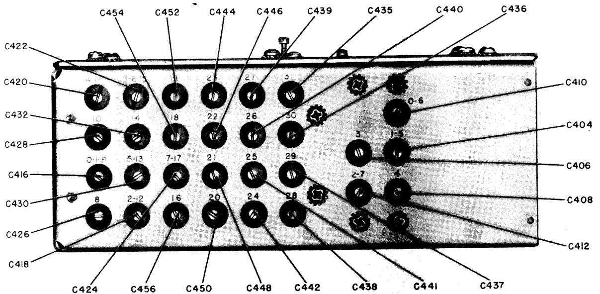
Figure 47. Crystal oscillator subchassis, top view.
