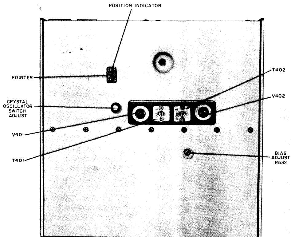
Figure 64. Receiver, rear view, case removed.
