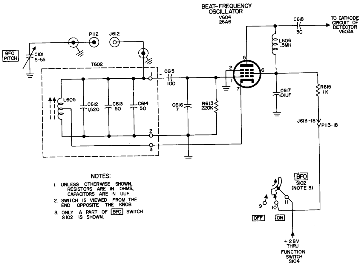
Figure 13. Beat-frequency oscillator, simplified schematic diagram.
