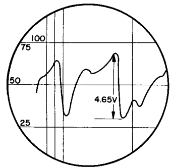
(J) WAVEFORM AT GRID PIN 7, V703
