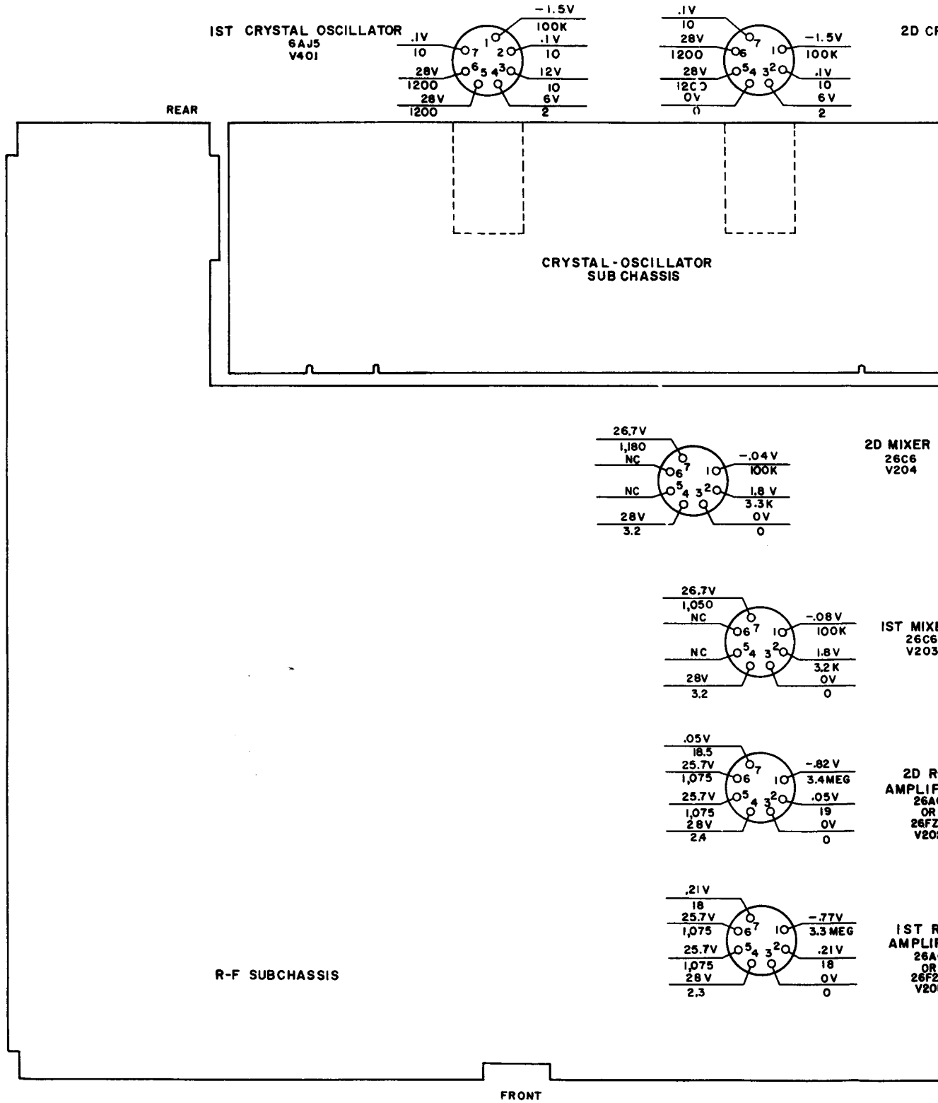
Figure 78. Upper deck, voltage and resistance
