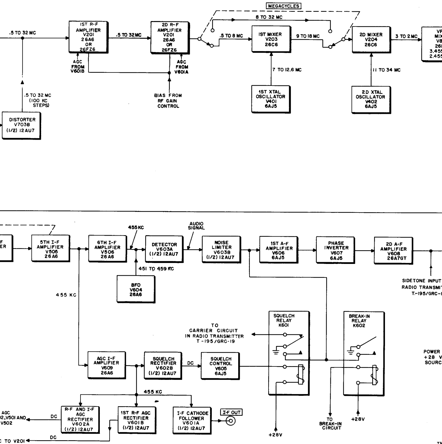
Figure 1. Radio Receiver R-392/URR, block diagram.
