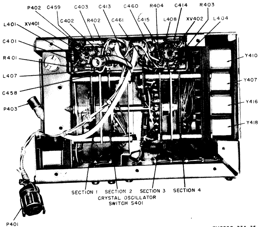
Figure 46. Crystal oscillator subchassis, front view, cover removed.
