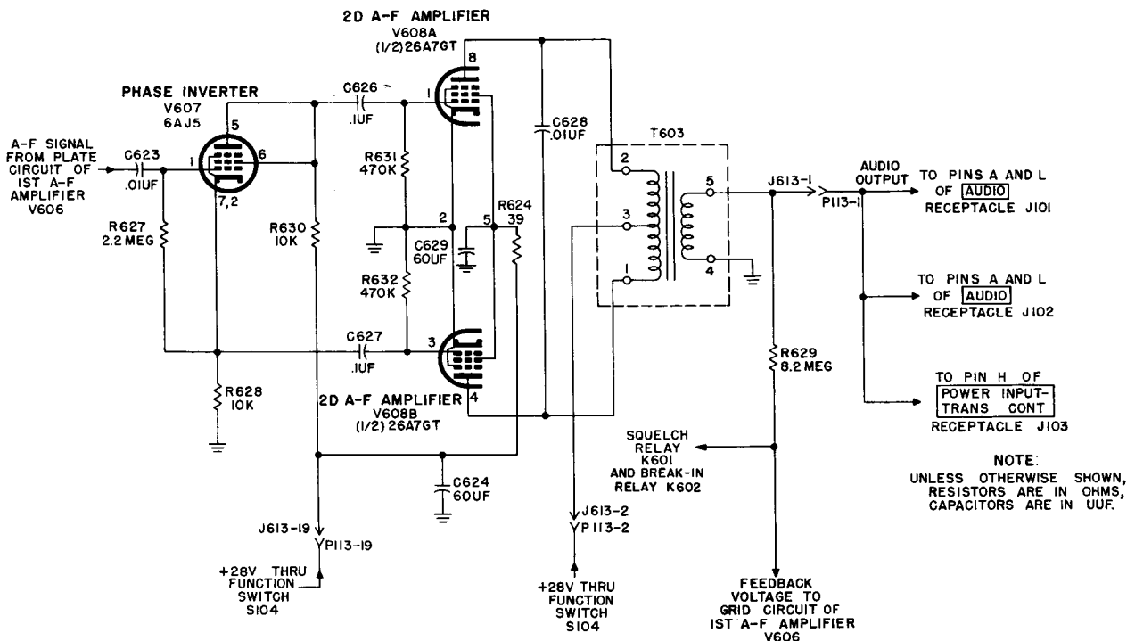
Figure 19. Phase inverter V607 and second audiofrequency amplifier V608, simplified schematic diagram.
