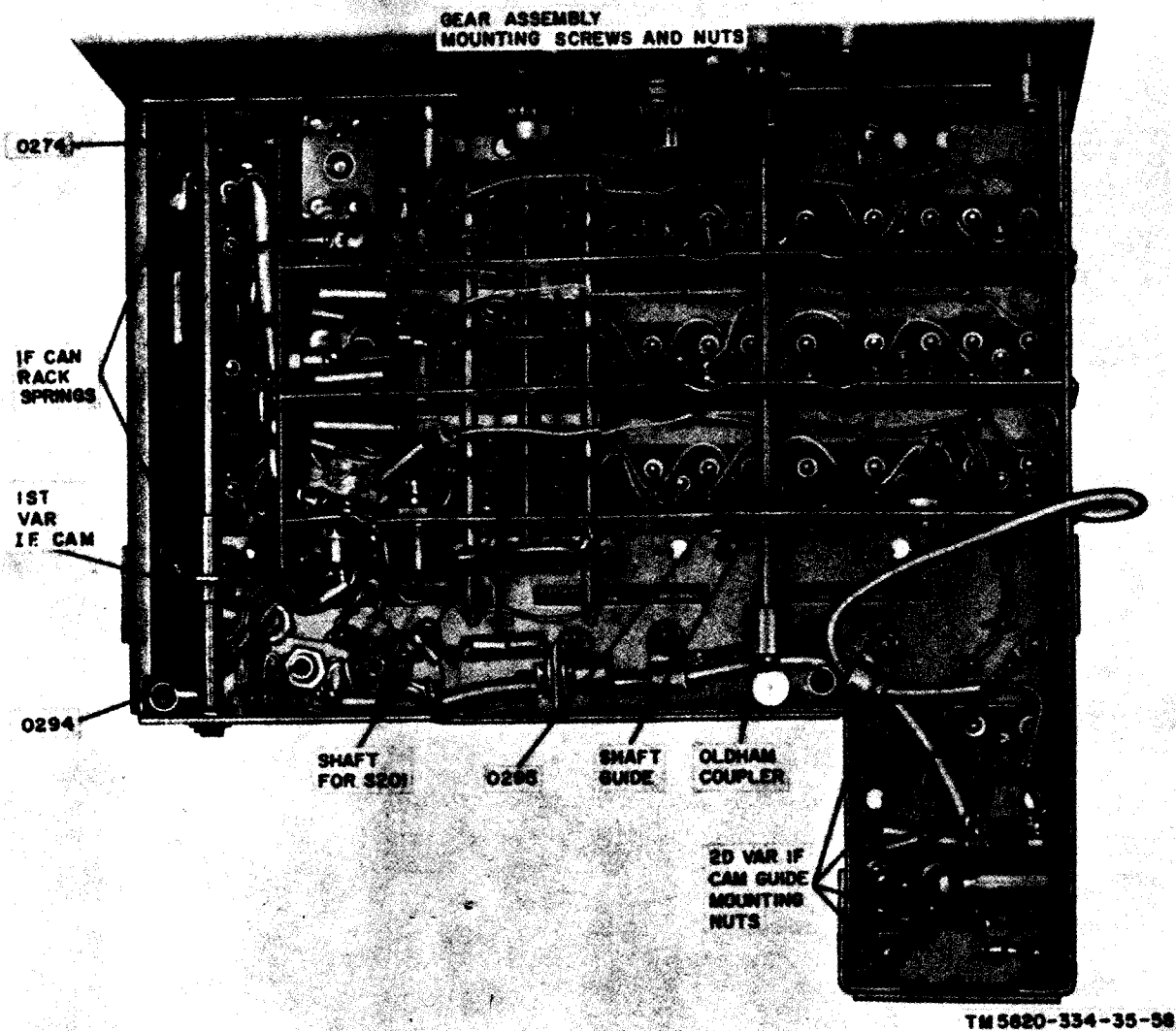
Figure 60. Rf subchassis, bottom view.
