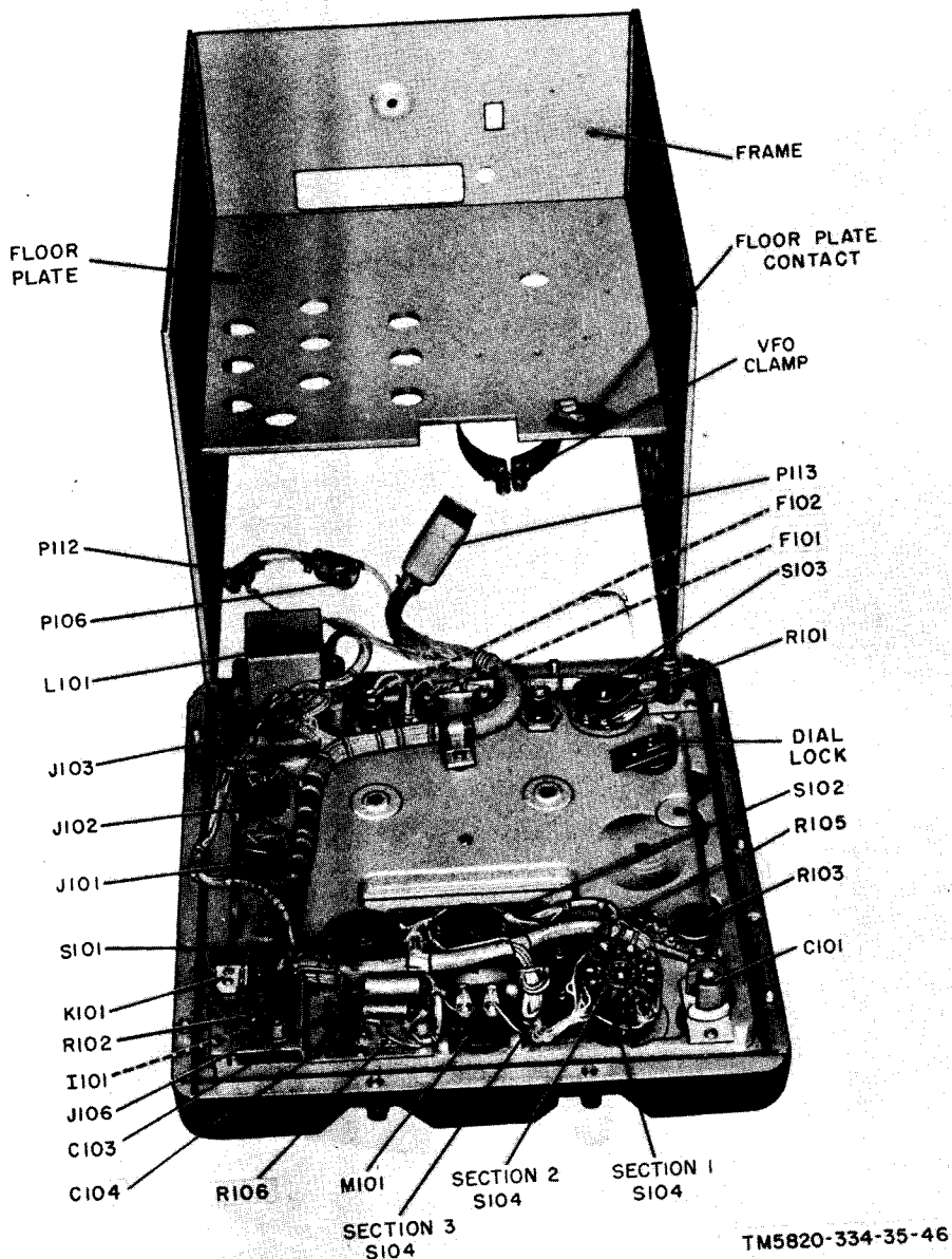
Figure 55. Front panel assembly, rear view.
