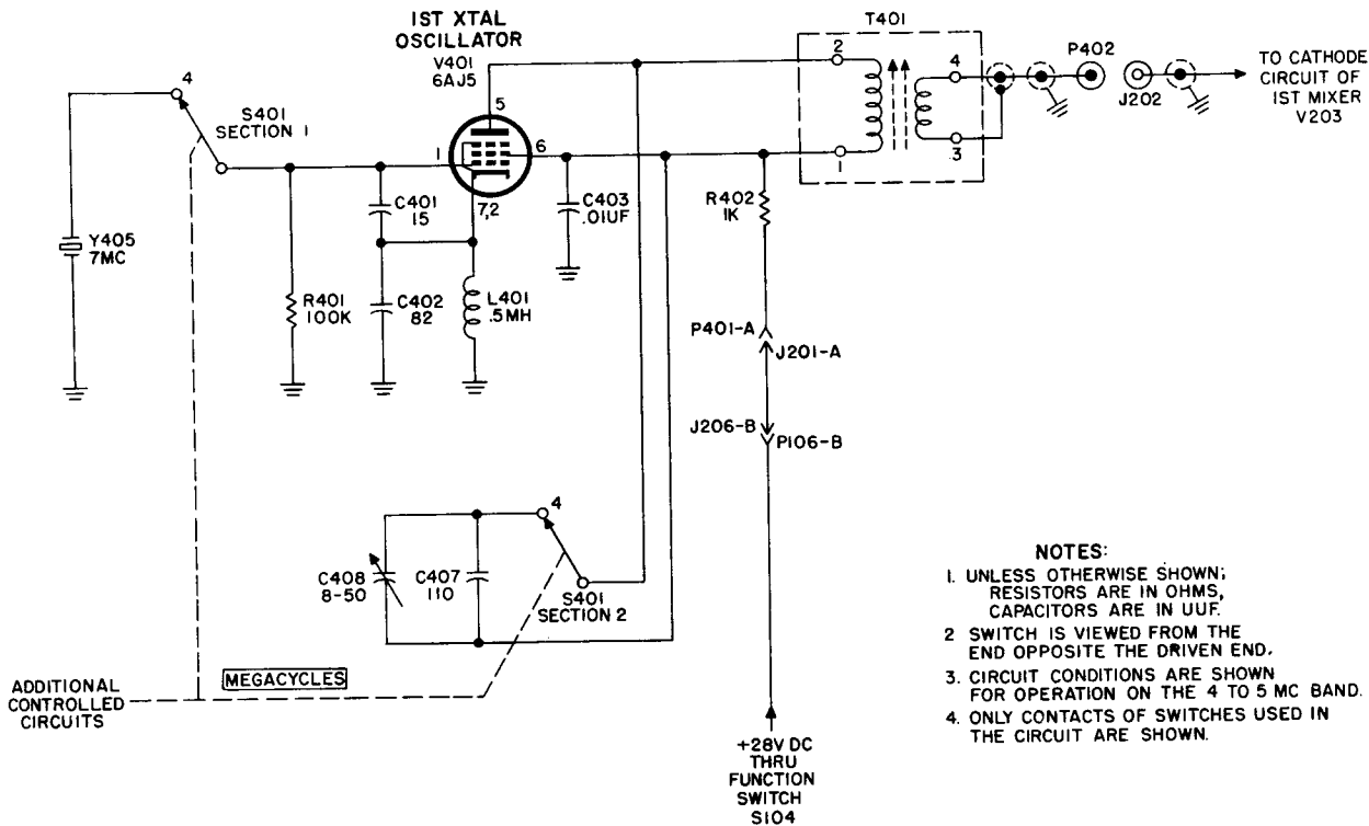
Figure 5. First crystal oscillator, simplified schematic diagram.
