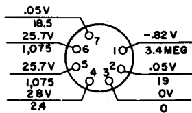
2D R-F AMPLIFIER 26A6 OR 26F26 V202
