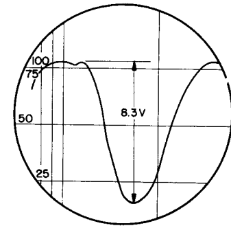
(F) WAVEFORM AT PLATE PIN 6, V701
