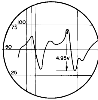
(H) WAVEFORM AT PLATE PIN 1, V703
