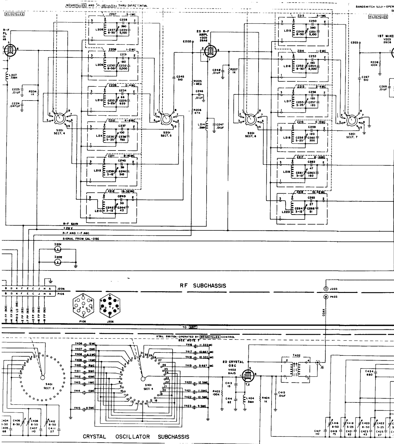
Figure 88(1). Radio receiver, wiring diagram (part 1 of 2).
