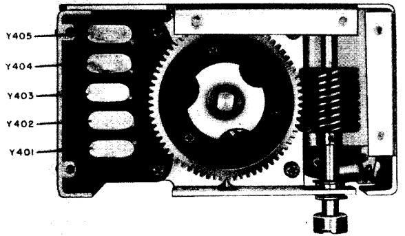
Figure 49. Crystal oscillator subchassis, right side view, cover removed.
