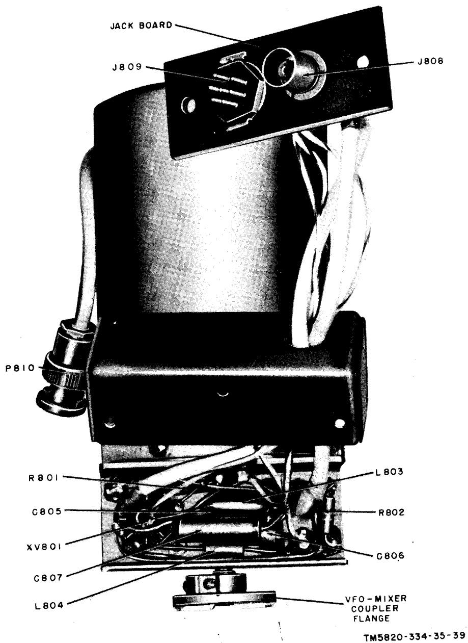
Figure 42. Vfo subchassis, bottom cover removed.
