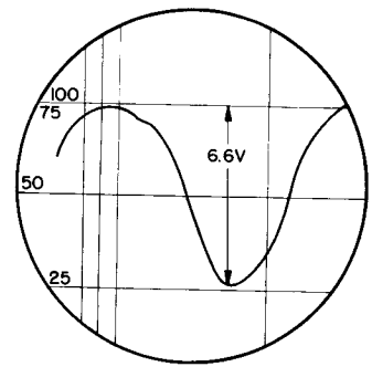
(C) WAVEFORM AT GRID PIN 2, V701
