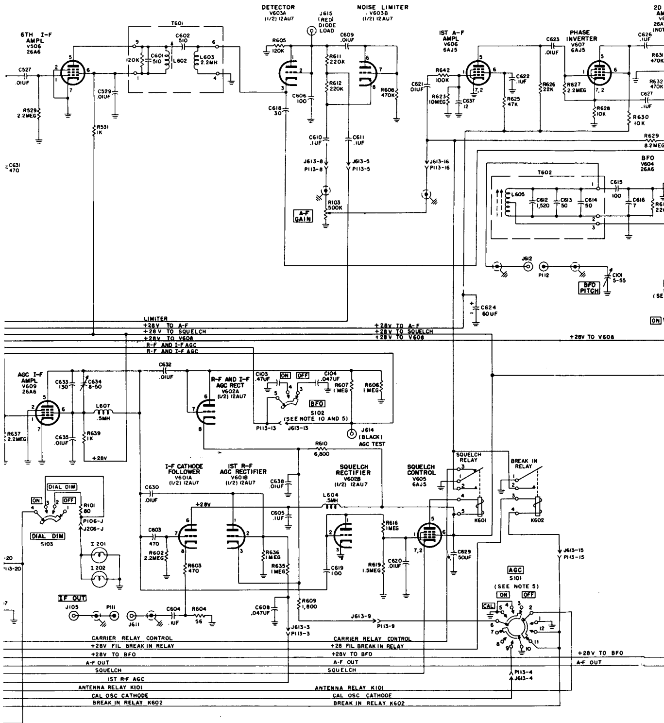
ceiver, schematic diagram (part 2 of 2).
