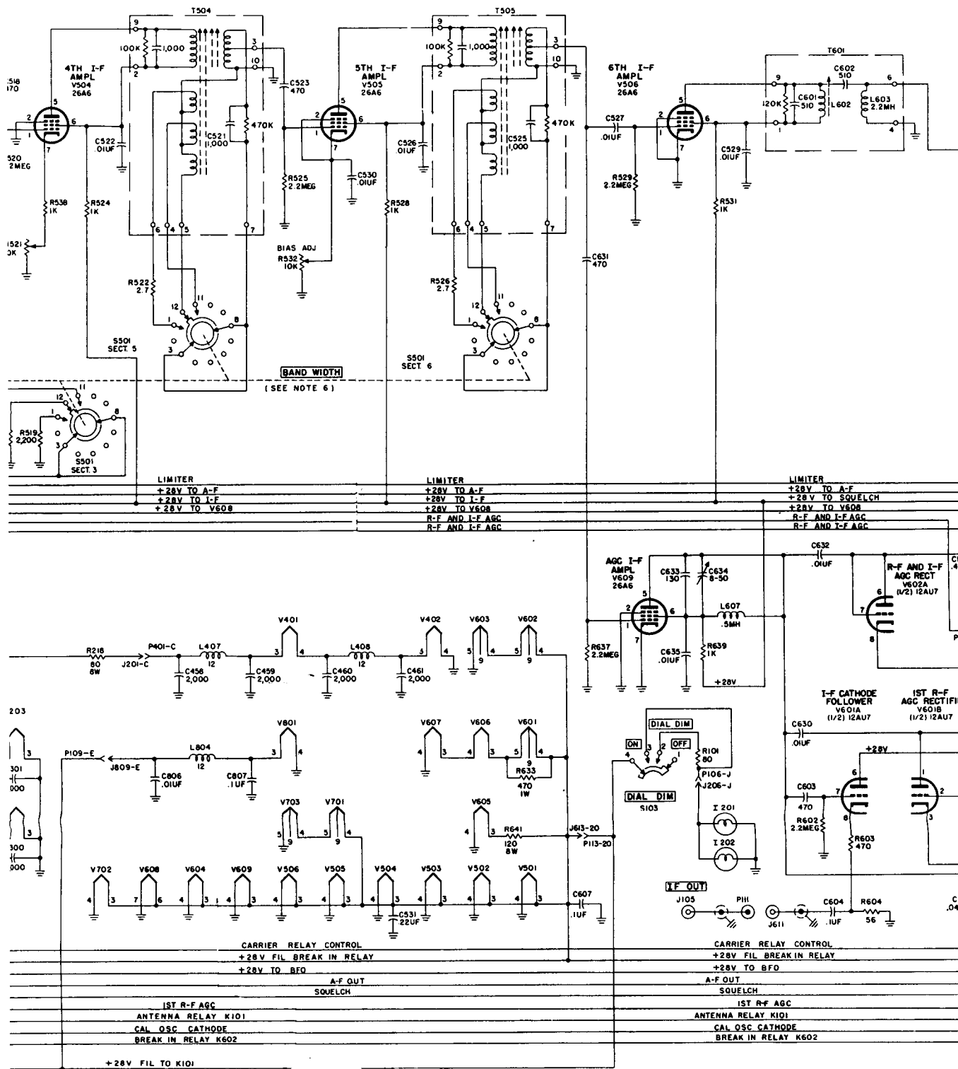
Figure 81(2). Radio receiver, schematic diagram (part 2 of 2).
