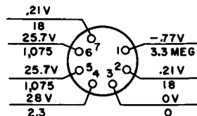
1ST R-F AMPLIFIER 26A6 OR 26F26 V201
